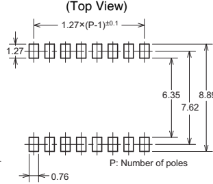
Dimensions of PCB pad (Reference)
