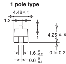
Flat actuator Standard
