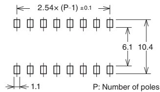
Dimensions of PCB pad (Reference) (Top View)
