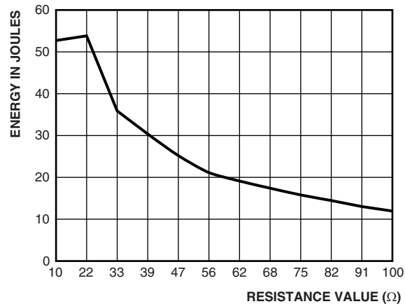
PULSE ENERGY CURVE FOR AC05-CS (1.2 / 50 μs; 10 pulses at 30 s interval)
