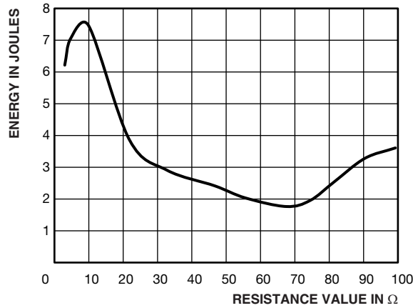
PULSE ENERGY CURVE FOR AC01-CS (1.2 / 50 μs; 10 pulses at 30 s interval)
