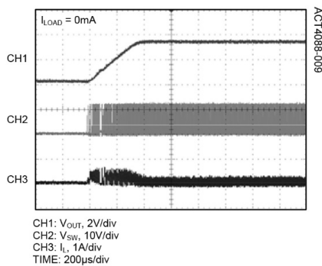
Start-up Waveforms
