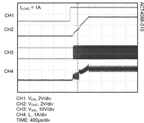
Start-up Waveforms
