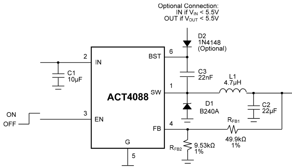
Figure 2: ACT4088 Typical 5V/1.5A Output Application
