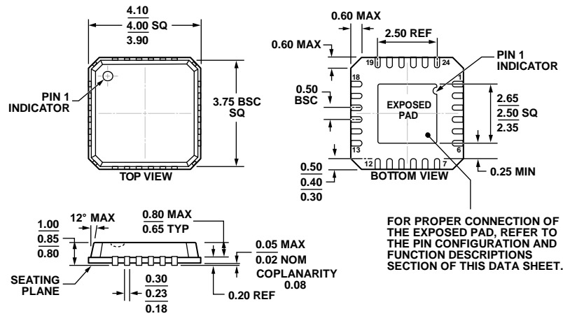
Figure 105. 24-Lead Lead Frame Chip Scale Package [LFCSP_VQ] 4 mm × 4 mm Body, Very Thin Quad (CP-24-3) Dimensions shown in millimeters
