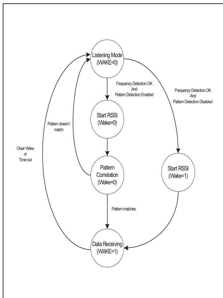
Figure 20: Operating Modes Flow Chart
