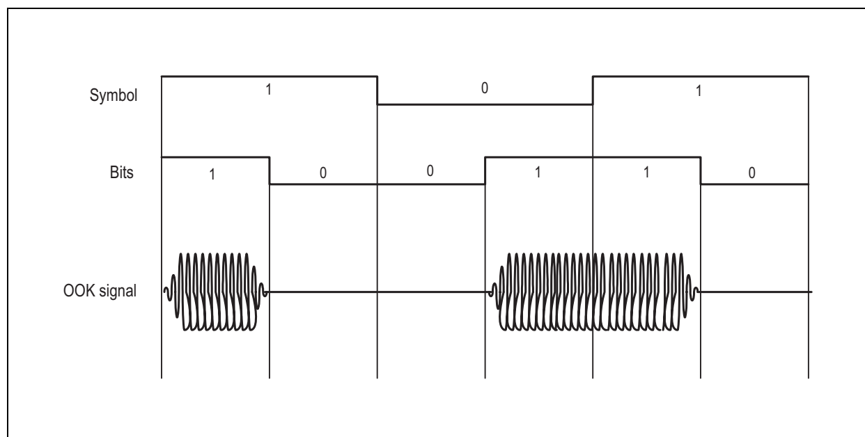
Figure 47: Manchester Encoding
