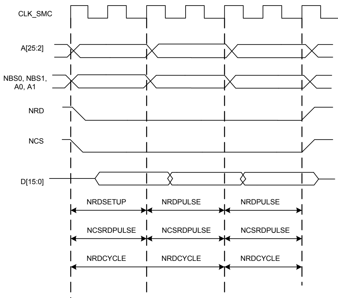
Figure 27-10. No Setup, No Hold on NRD, and NCS Read Signals
