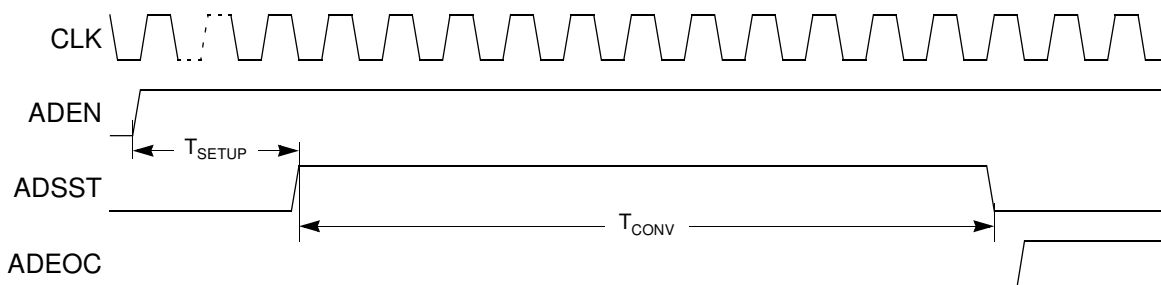
Figure 39. Timing Diagram
