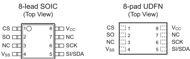
Figure 8-1. Pin Configurations
