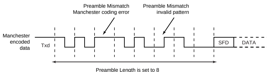
Figure 34-16. Manchester Error Flag
