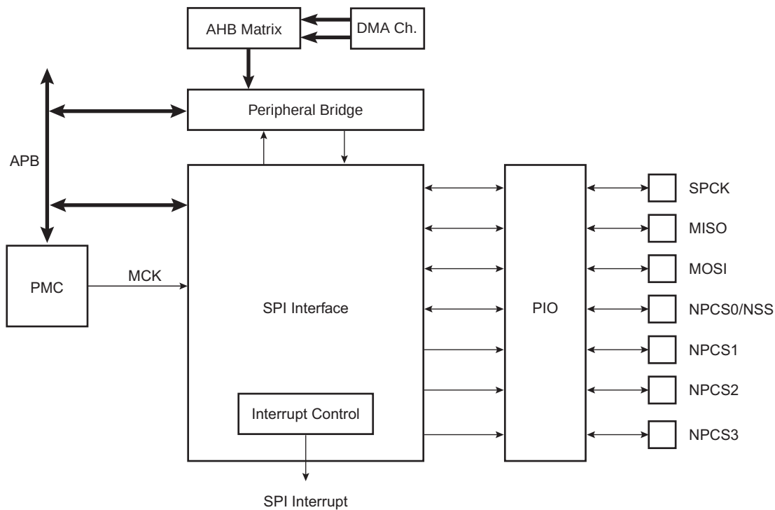
Figure 31-1. Block Diagram
