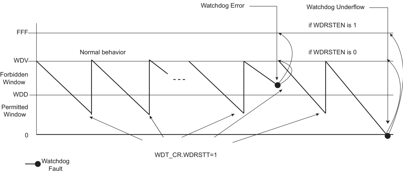
Figure 17-2. Watchdog Behavior
