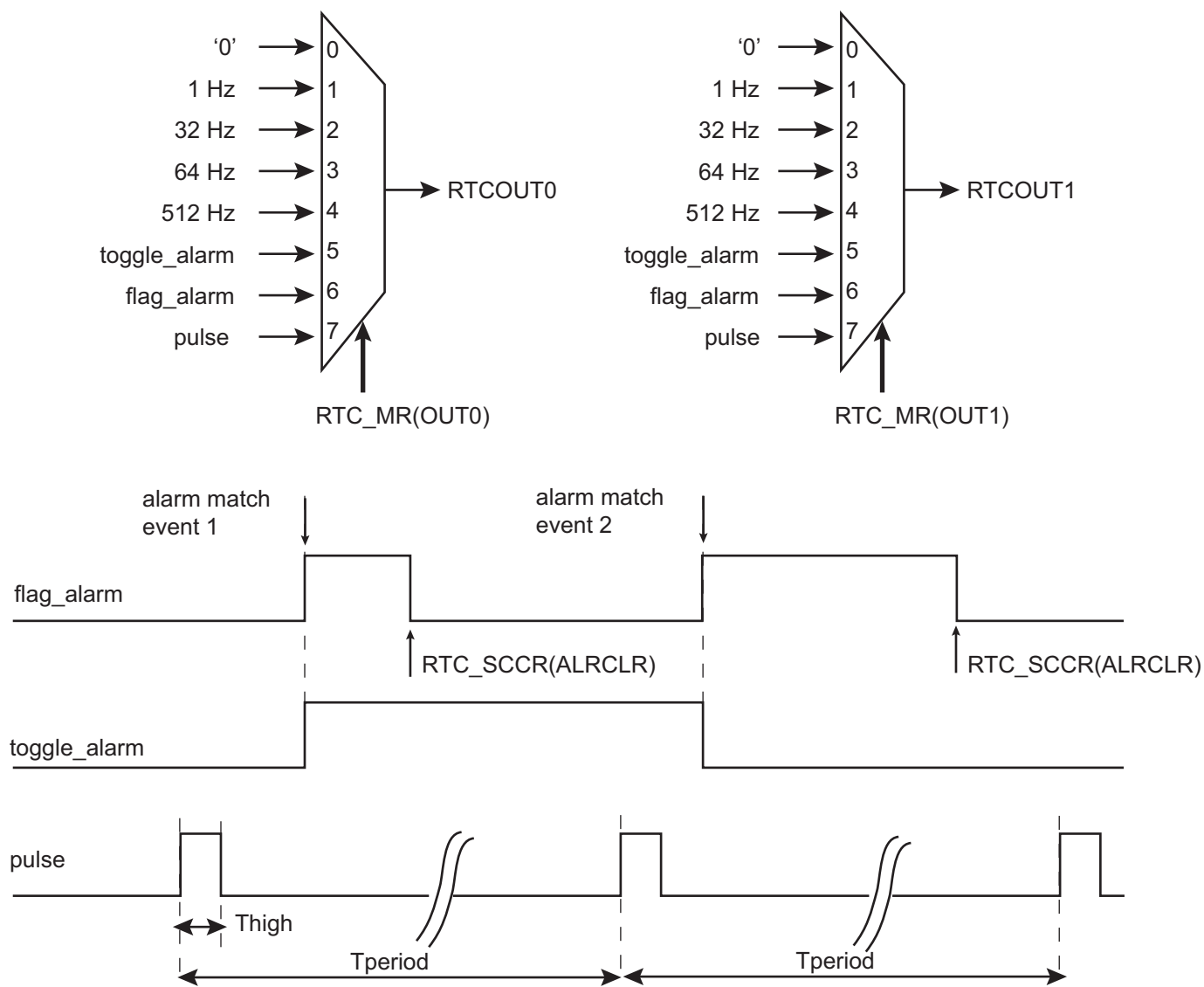
Figure 16-5. Waveform Generation
