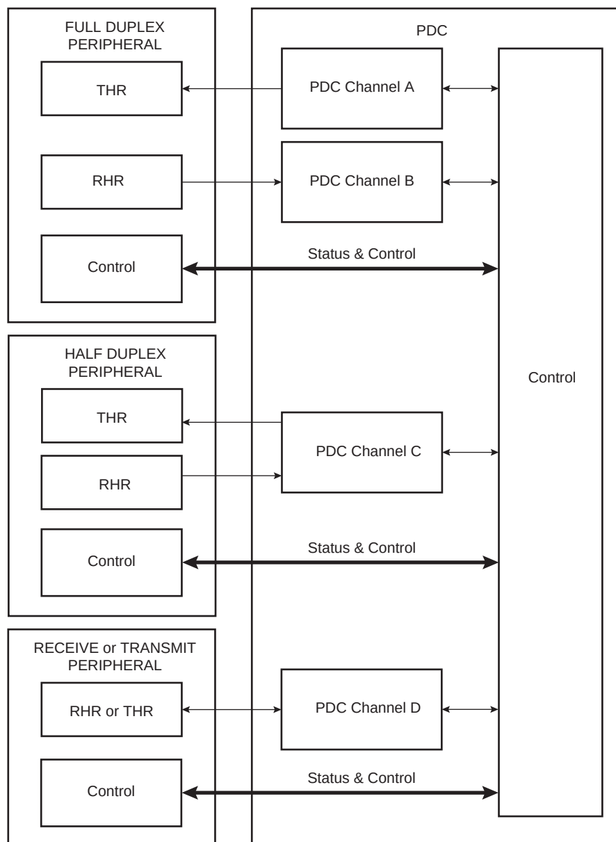
Figure 27-1. Block Diagram
