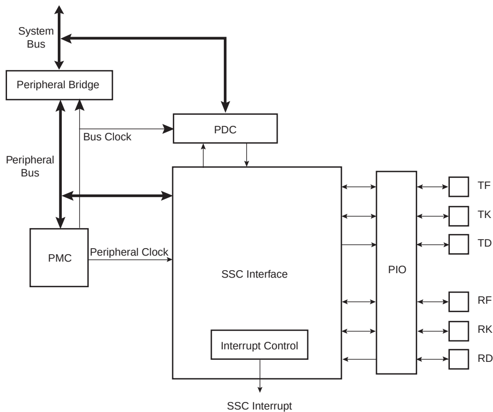
Figure 32-1. Block Diagram
