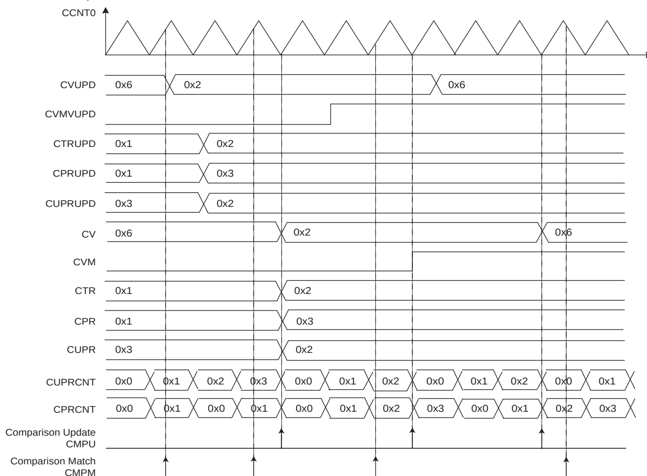
Figure 39-15. Comparison Waveform
