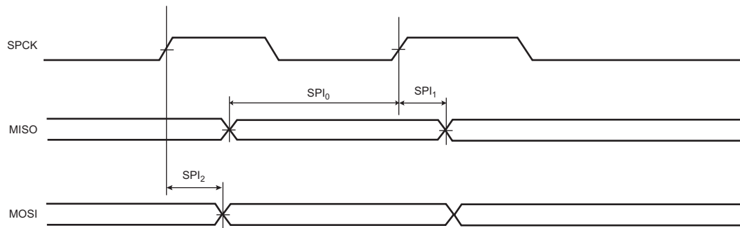
Figure 44-22. SPI Master Mode with (CPOL = NCPHA = 0) or (CPOL = NCPHA = 1)
