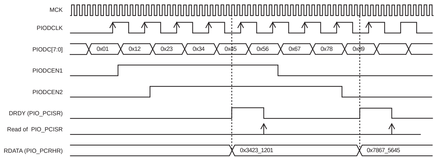
Figure 31-10. Parallel Capture Mode Waveforms (DSIZE = 2, ALWAYS = 1, HALFS = 0)
