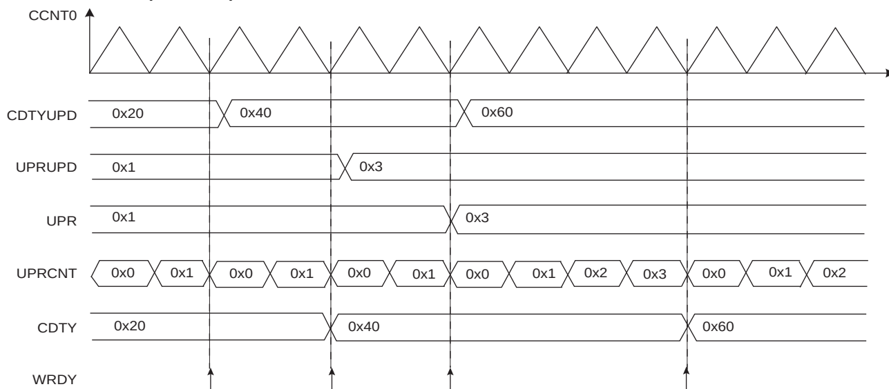
Figure 39-11. Method 2 (UPDM = 1)
