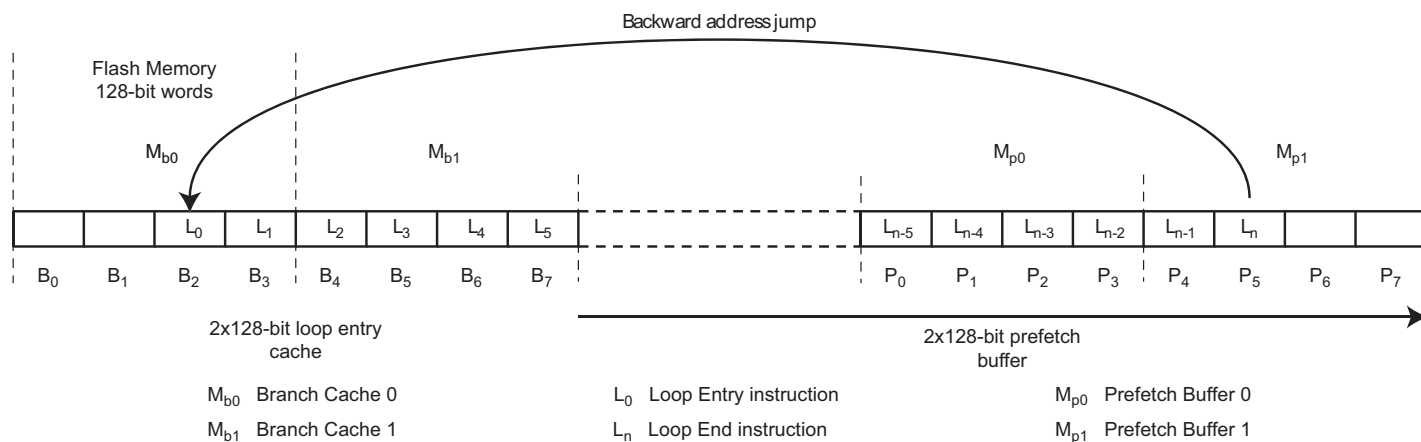
Figure 20-5. Code Loop Optimization
