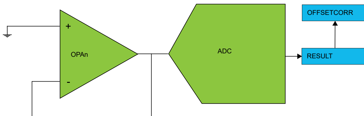
Figure 41-12. Offset Compensation
