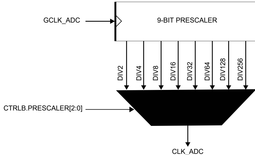
Figure 42-2. ADC Prescaler
