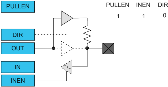
Figure 29-5. I/O Configuration - Input with Pull
