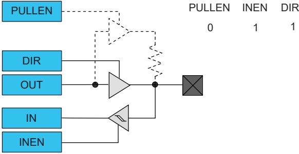
Figure 29-7. I/O Configuration - Totem-Pole Output with Enabled Input
