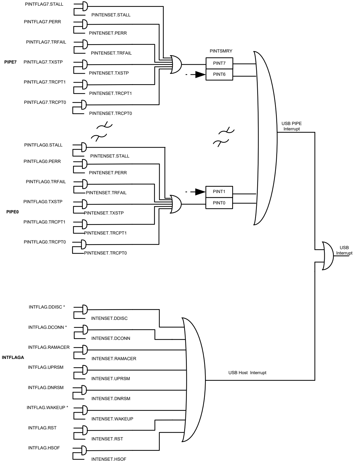
Figure 39-10. Host Interrupt
