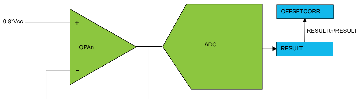
Figure 41-13. Gain Compensation
