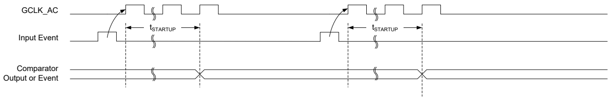
Figure 43-10. Single-Shot SleepWalking
