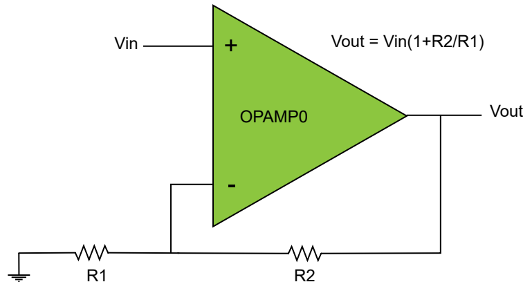
Figure 41-4. Non-Inverting PGA
