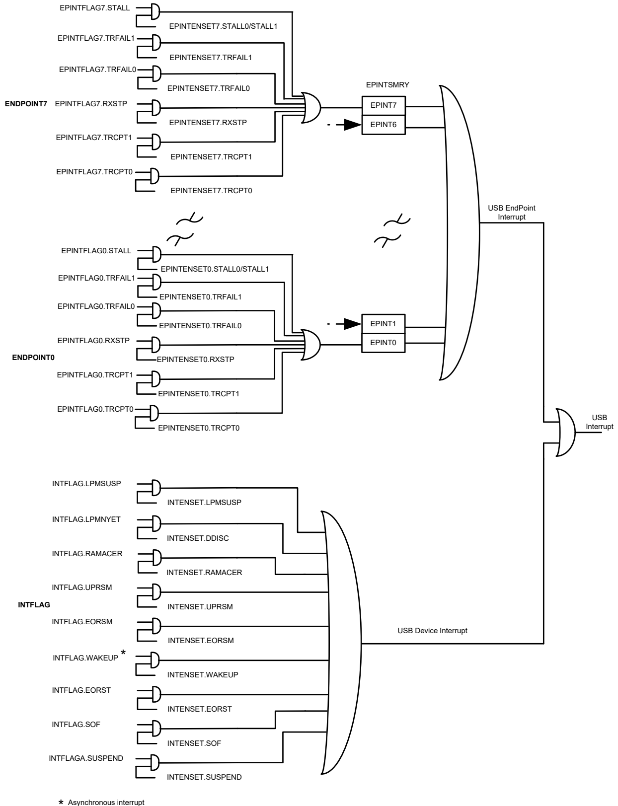
Figure 39-9. Device Interrupt
