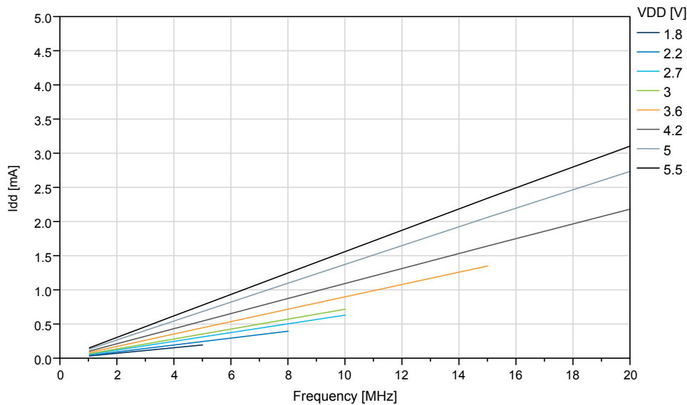
Figure 35-6. ATtiny416: Idle Supply Current vs. Frequency (1-20MHz) at T=25^{\circ}\text{C}
