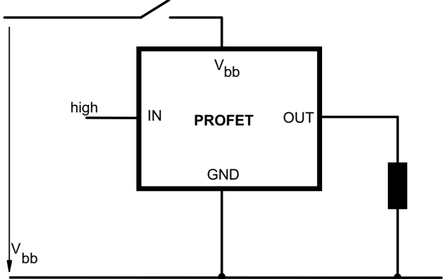
V bb disconnect with charged inductive load
