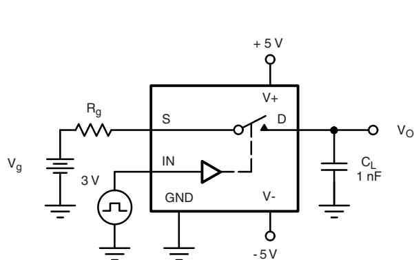
Fig. 3 - Charge Injection
