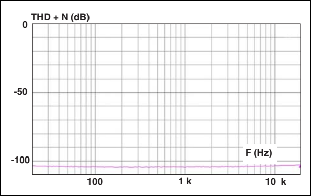
Figure 13. Total harmonic distortion with noise: EAR lines, R = 32\text{ }\Omega
