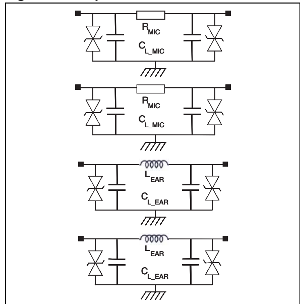
Figure 2. Equivalent circuit
