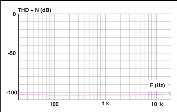
Figure 14. Total harmonic distortion with noise: EAR lines, R = 8\text{ }\Omega
