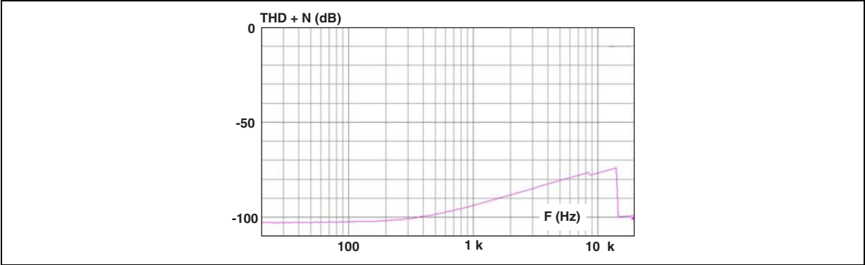
Figure 14. Total harmonic distortion with noise: EAR lines, R = 8\text{ }\Omega
