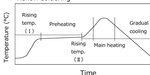
Reflow soldering
