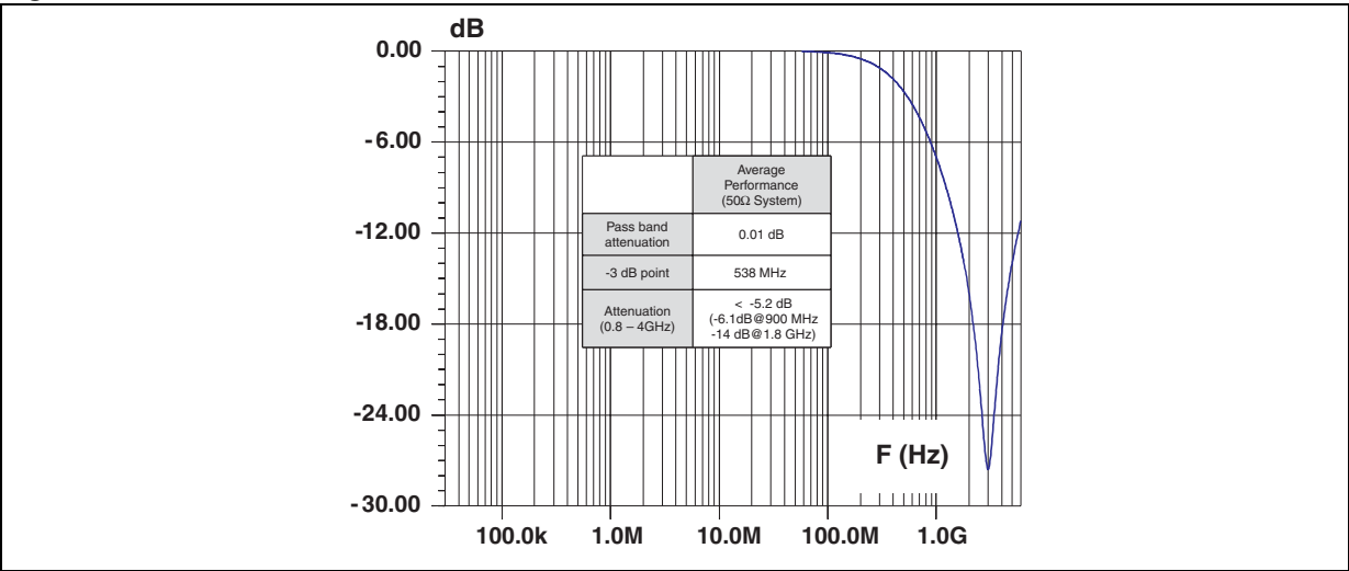
Figure 10. S21 attenuation measurement results
