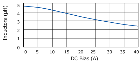
[ ETQP6M4R7YLC ]
