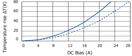
[ ETQP6M2R5YLC ]
