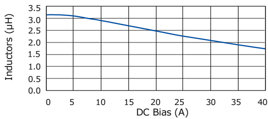
[ ETQP6M3R3YLC ]
