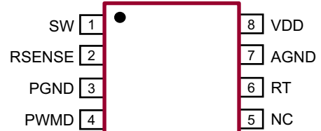
8-Lead MSOP (MG) (top view)
