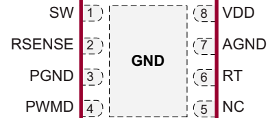
8-Lead DFN (K7) (top view)
