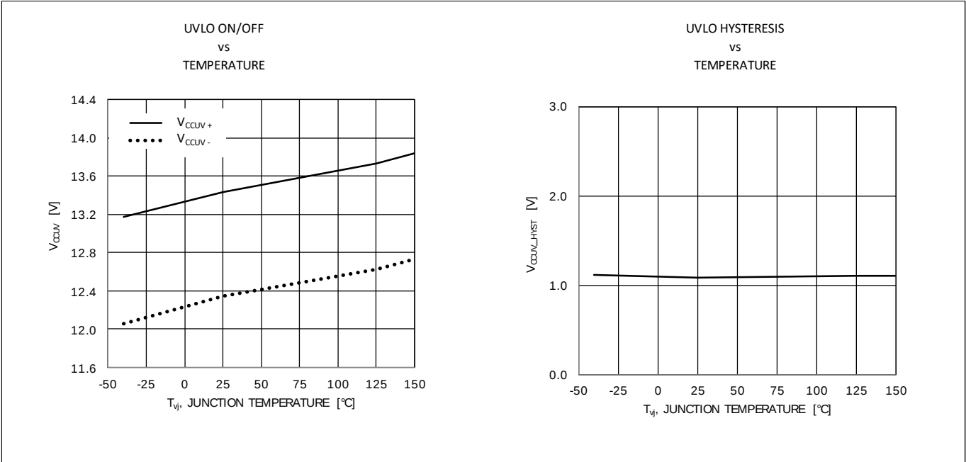
Figure 12. Undervoltage Lockout
