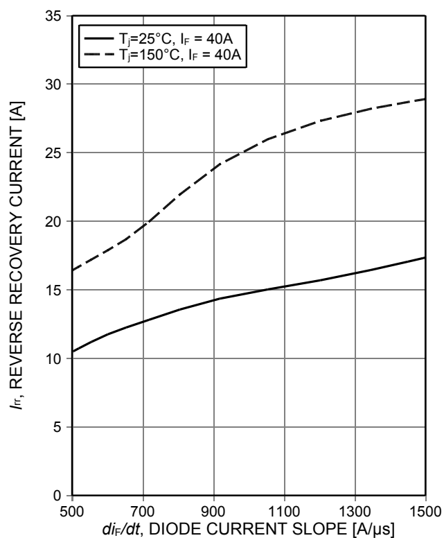
Figure 21. Typical reverse recovery current as a function of diode current slope ( V_R=400\text{V} )
