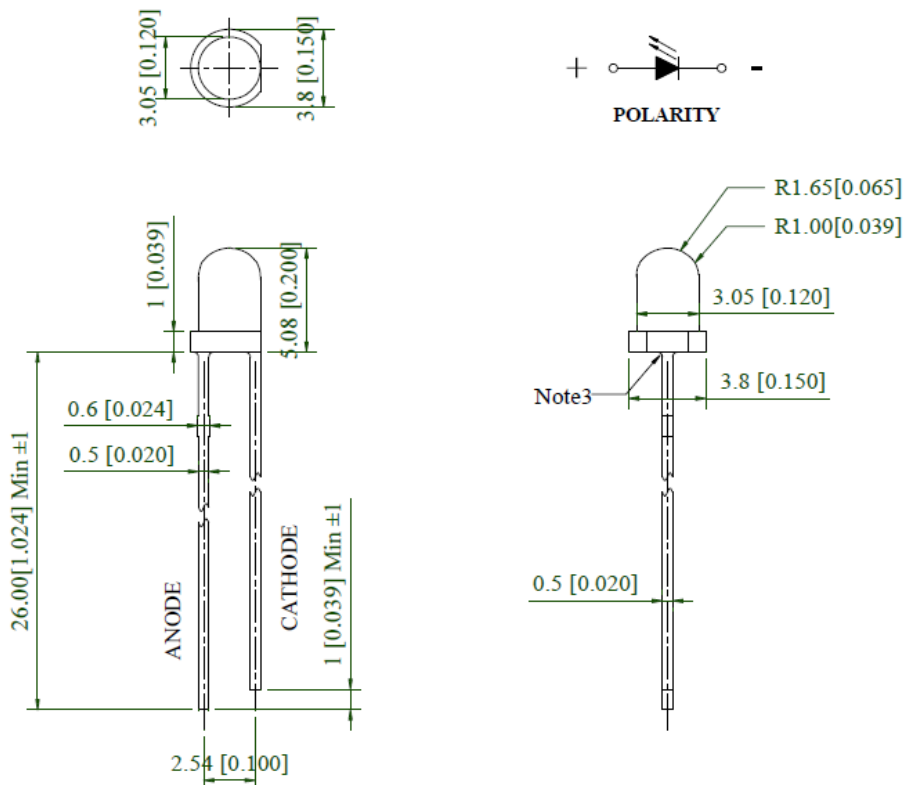
Figure 1. INL-3AX30 Package Dimensions
