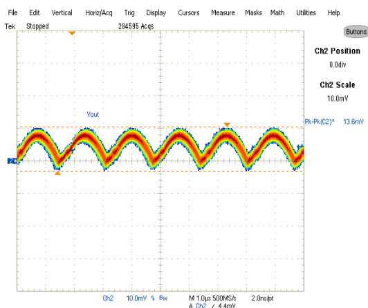
Fig. 20: Output Voltage Ripple, 8A load Ch 2 : V_{out}
