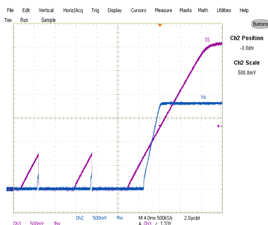
Fig. 22: Short (Hiccup) Recovery Ch 2 : V_{out} , Ch 3 : V_{ss}
