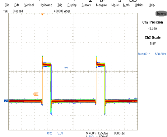
Fig. 21. Inductor node at 4A load Ch2: LX
