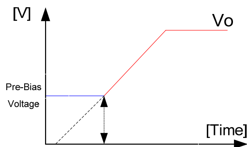
Fig. 4. Pre-Bias startup
