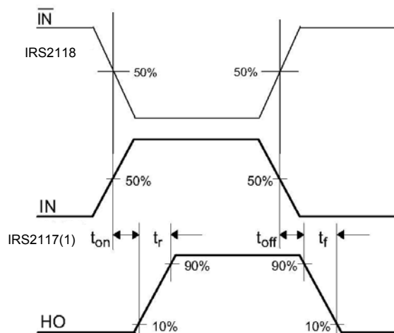
Figure 4 Switching Time Waveform Definition
