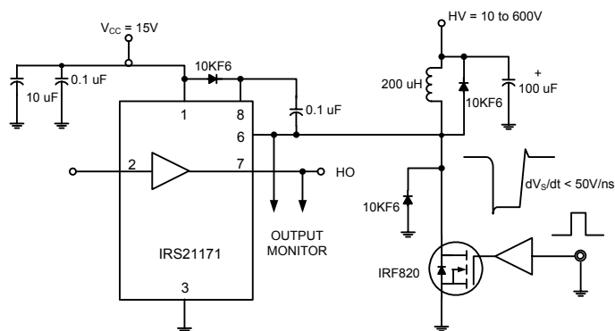
Figure 2 Floating Supply Voltage Transient Test
