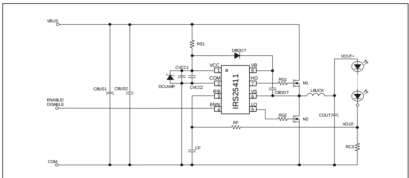
Figure 1 Typical schematic
