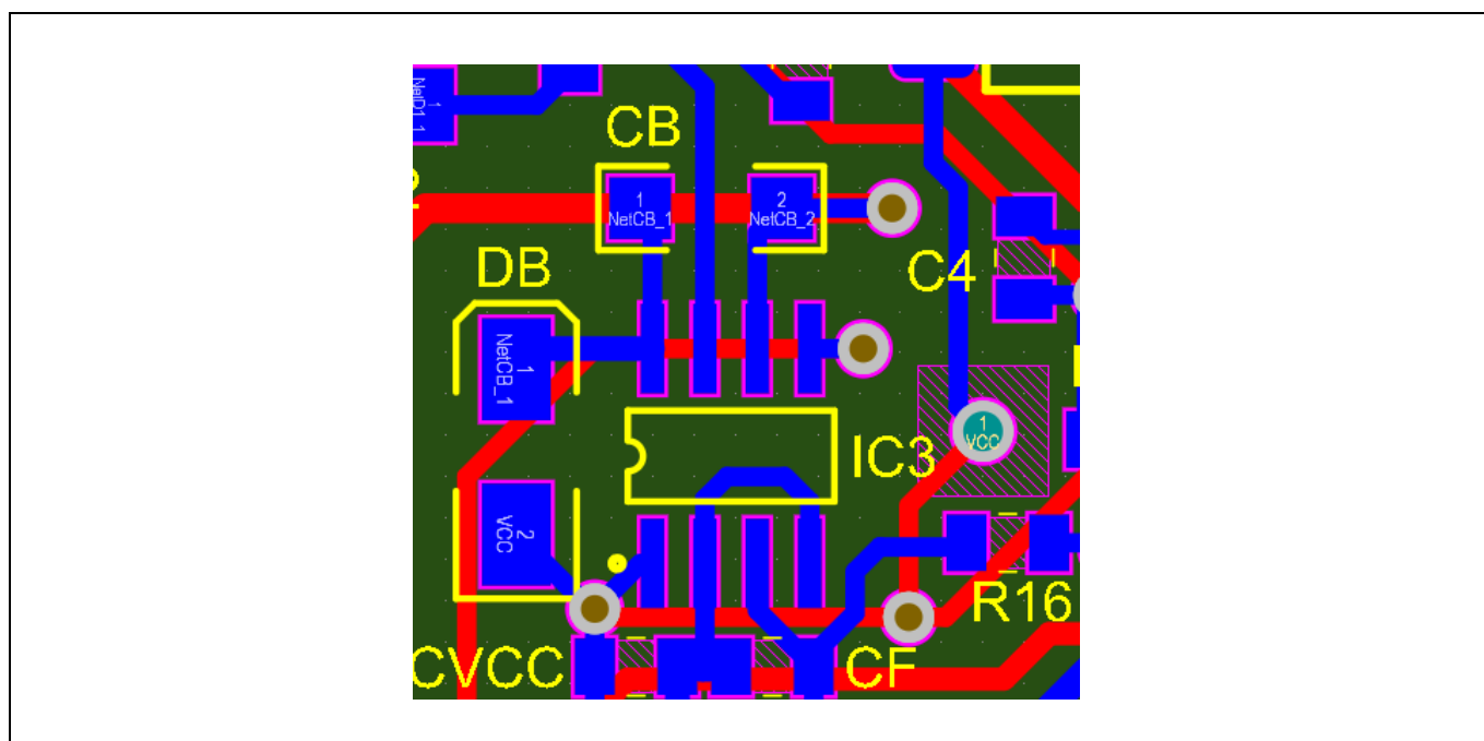
Figure 11 IRS25411 correct layout example
