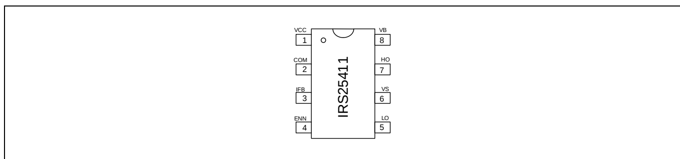
Figure 3 Pin assignments
