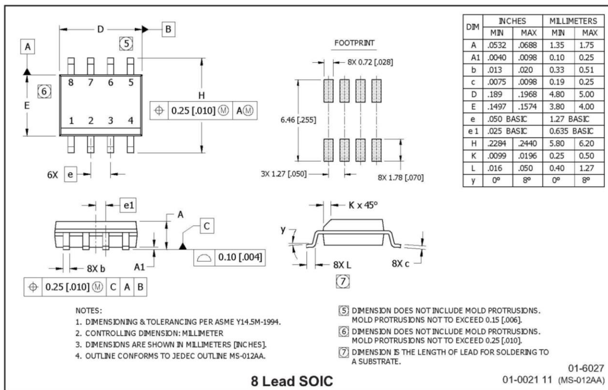
Figure 12 Package details
