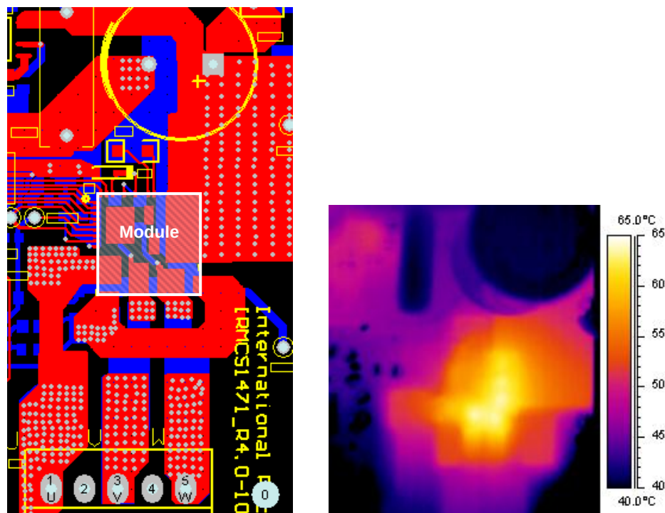
Figure 7: PCB layout example and corresponding thermal image (6kHz, 2P, 2oz, \Delta T_{ca}=40^\circ\text{C} , V_+ = 150\text{V} , I_u = 427\text{mA}_{rms} , P_o = 94\text{W} )
