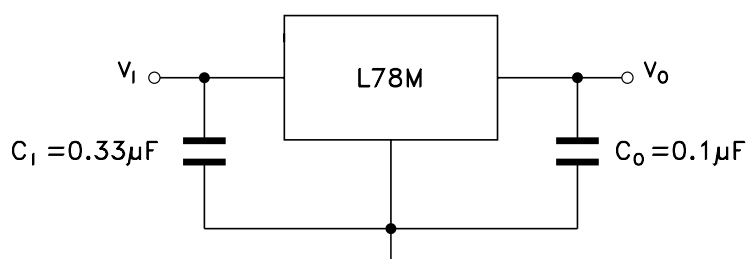
Figure 4. Application circuit
