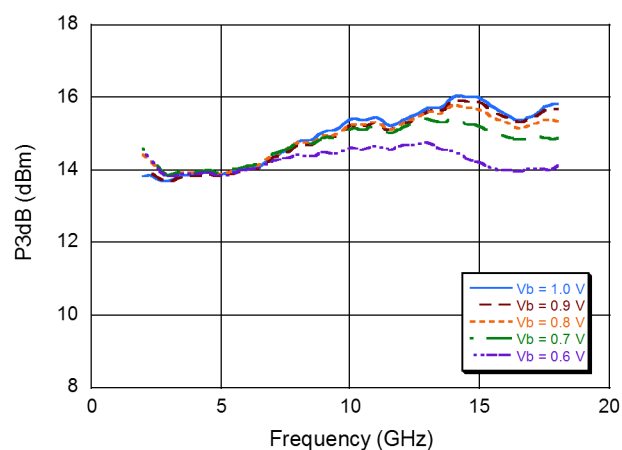
P3dB @ T_A = 25^\circ\text{C} , V_{DD} = 5\text{ V}
