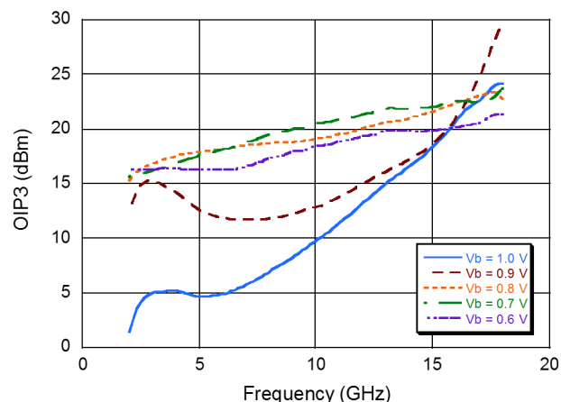
Output IP3 @ T_A = -40^\circ\text{C} , V_{DD} = 3.3\text{ V}
