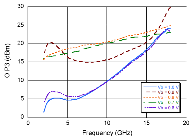
Output IP3 @ T_A = 85^\circ\text{C} , V_{DD} = 3.3\text{ V}
