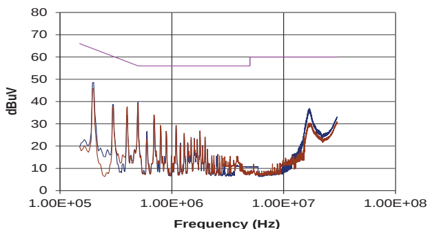
MGJ6D12XXXXWMC (Quasi-Peak)
