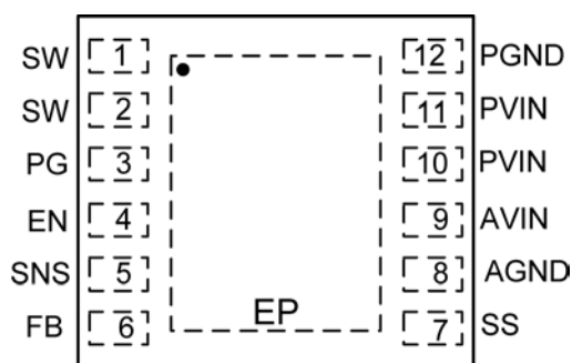
3mm x 3mm DFN (ML) (Top View)
