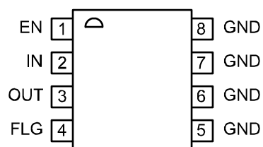
MIC5216-xxBMM/YMM MM8™ MSOP-8 Fixed Voltages
