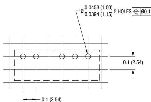
6 Pin SIP Package
