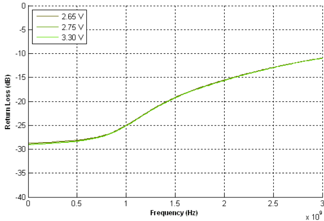
Figure 10. Return Loss at Active Port @ 25 °C
