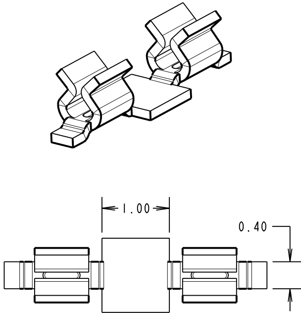
COMPONENT DETAILS
