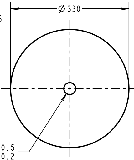
REEL DETAILS
