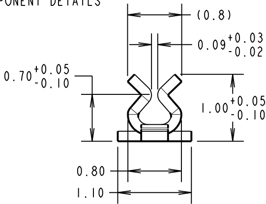
COMPONENT DETAILS
