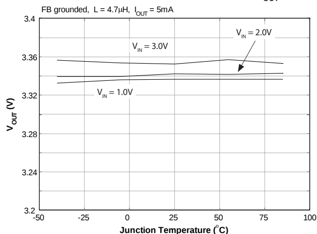
Temperature Regulation — PSAVE Mode ( V_{OUT} = 3.3V )
