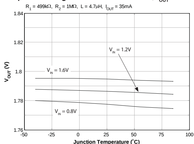
Temperature Regulation — PWM Mode ( V_{OUT} = 1.8V )
