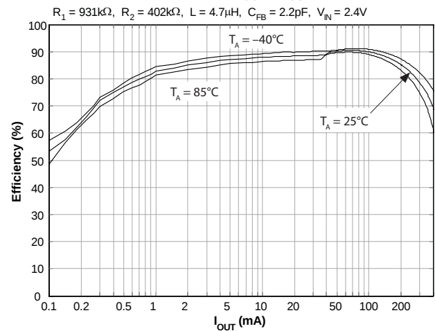
Efficiency vs. I_{OUT} ( V_{OUT} = 4.0V )
