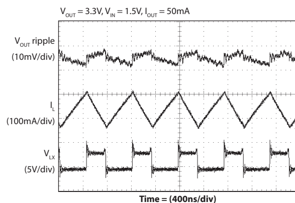
PWM Operation
