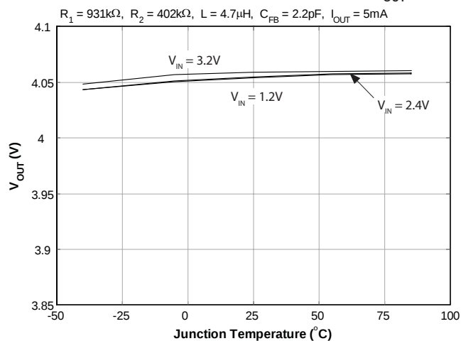
Temperature Regulation — PSAVE Mode ( V_{OUT} = 4.0V )
