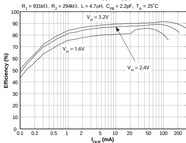
Efficiency vs. I_{OUT} ( V_{OUT} = 5.0V )
