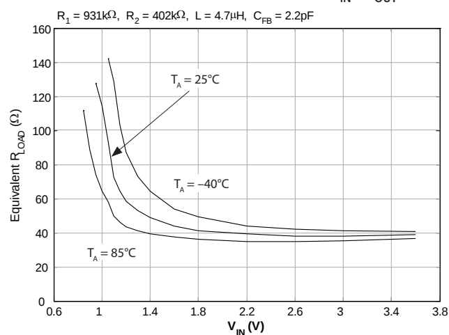
Startup Minimum Load Resistance vs. V_{IN} ( V_{OUT} = 4.0V )
