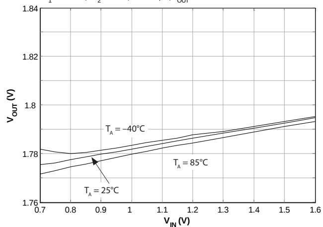
Line Regulation — PWM Mode ( V_{OUT} = 1.8V )
