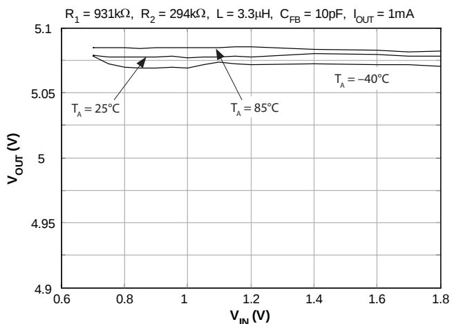
Line Regulation — PS/BAV Mode ( V_{OUT} = 5.0V )
