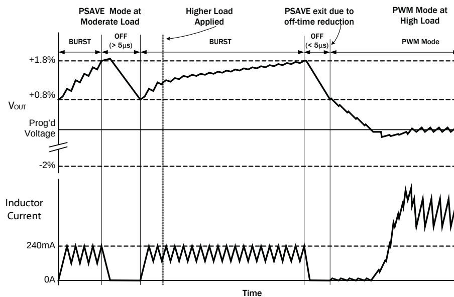
Figure 3 — PSAVE Operation With Exit to PWM Due To Off-time < 5µs
