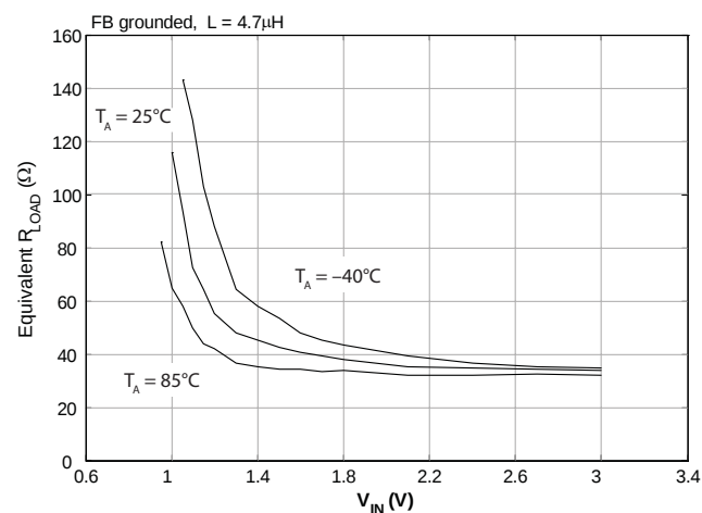
Startup Minimum Load Resistance vs. V_{IN} ( V_{OUT} = 3.3V )
