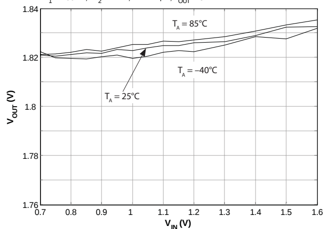
Line Regulation — PS/BAV Mode ( V_{OUT} = 1.8V )
