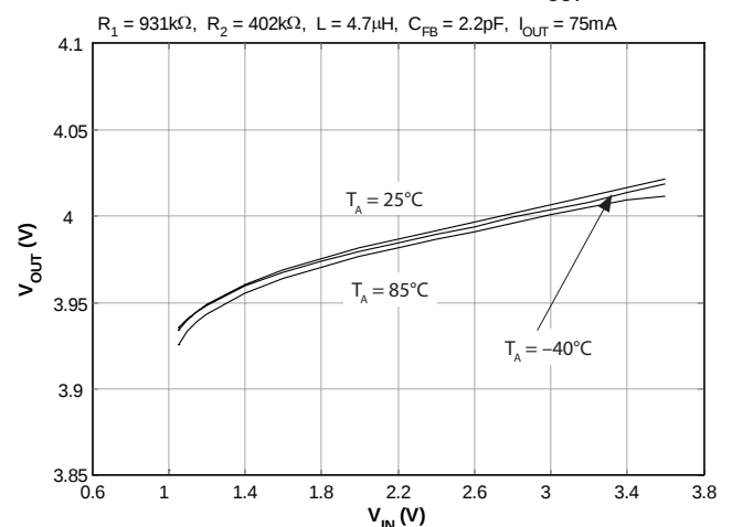
Line Regulation — PWM Mode ( V_{OUT} = 4.0V )
