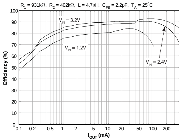
Efficiency vs. I_{OUT} ( V_{OUT} = 4.0V )
