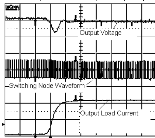
Load Transient Test ( V_{IN}=5V , V_{OUT}=1.2V , I_{OUT}= 0A to 4A , Forced Continuous Conduction Mode, L_{OUT}=1.3\mu H , C_{OUT}=3x22\mu F , Channel 1: 50mV/Div, Channel 2: 5V/Div, Channel 4: 2A/Div, Time: 10 \mu s /Div)
