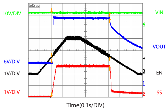
Start up and Shutdown by EN
