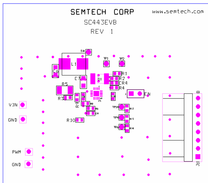
COMPONENT TOP
