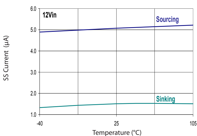
SS Current vs. Temperature
