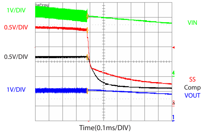
Shutdown by Vin
