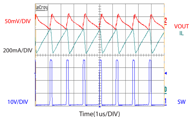
Main Power Switching Waveform
