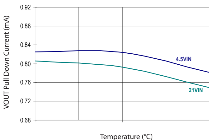
VOUT Pull Down Current vs. Temperature
