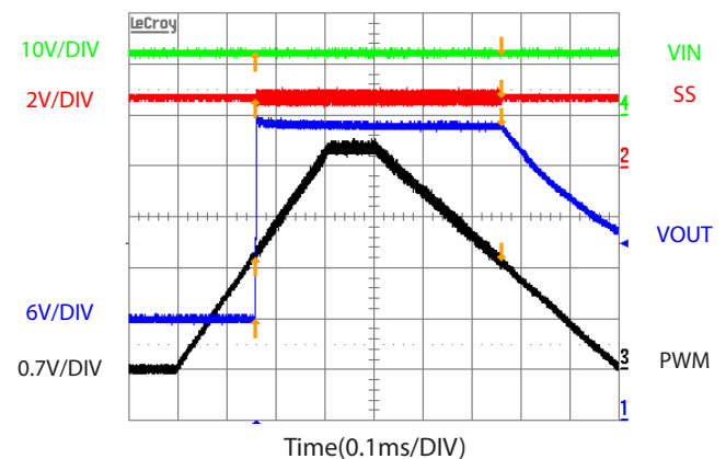
Start up and Shutdown by PWM
