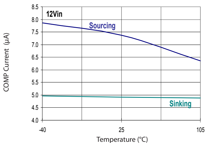
COMP Current vs. Temperature
