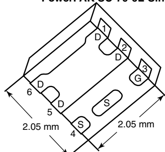
PowerPAK SC-70-6L-Single
