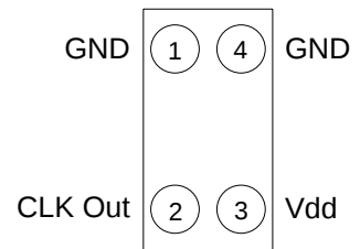
Figure 1. Pin Assignments
