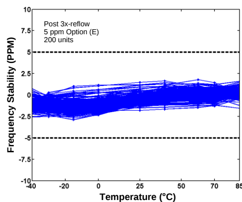
Figure 6. Frequency Stability Over Temperature (Post-Reflow)
