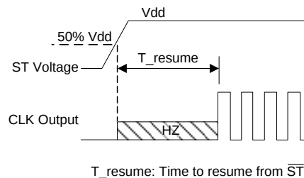
Figure 4. Standby Resume Timing ( \overline{\text{ST}} Mode Only)
