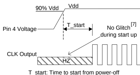
Figure 3. Startup Timing (OE/ \overline{\text{ST}} Mode)
