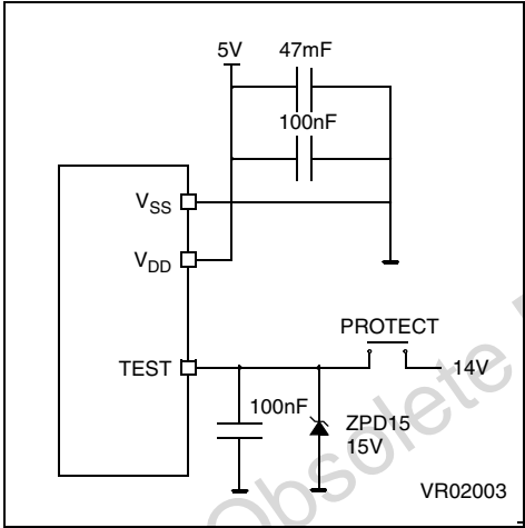
Figure 55. Programming Circuit
