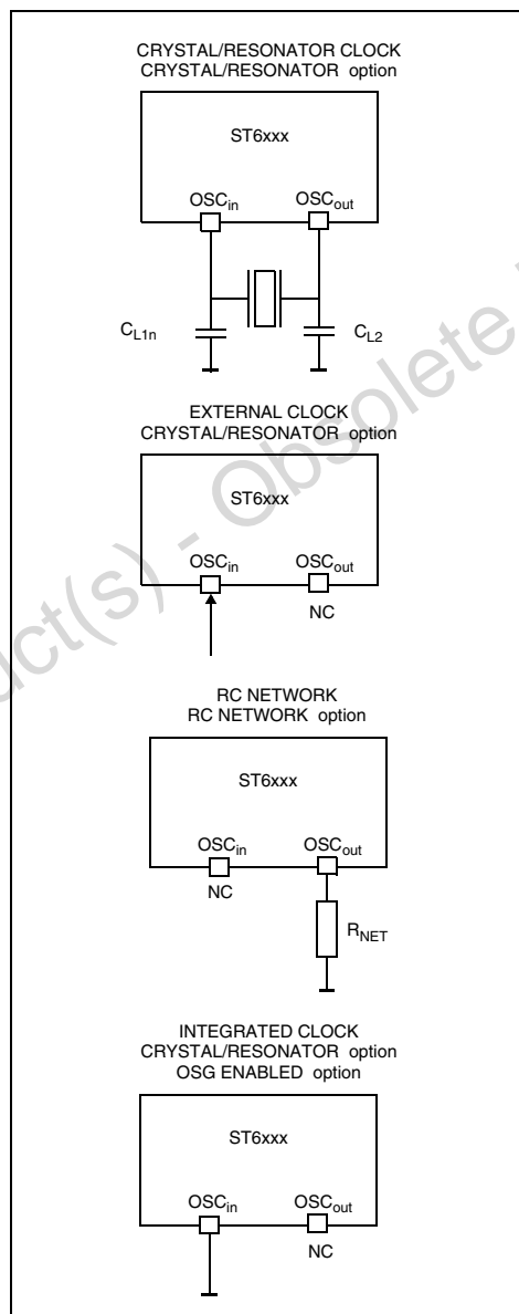
Figure 9. Oscillator Configurations
