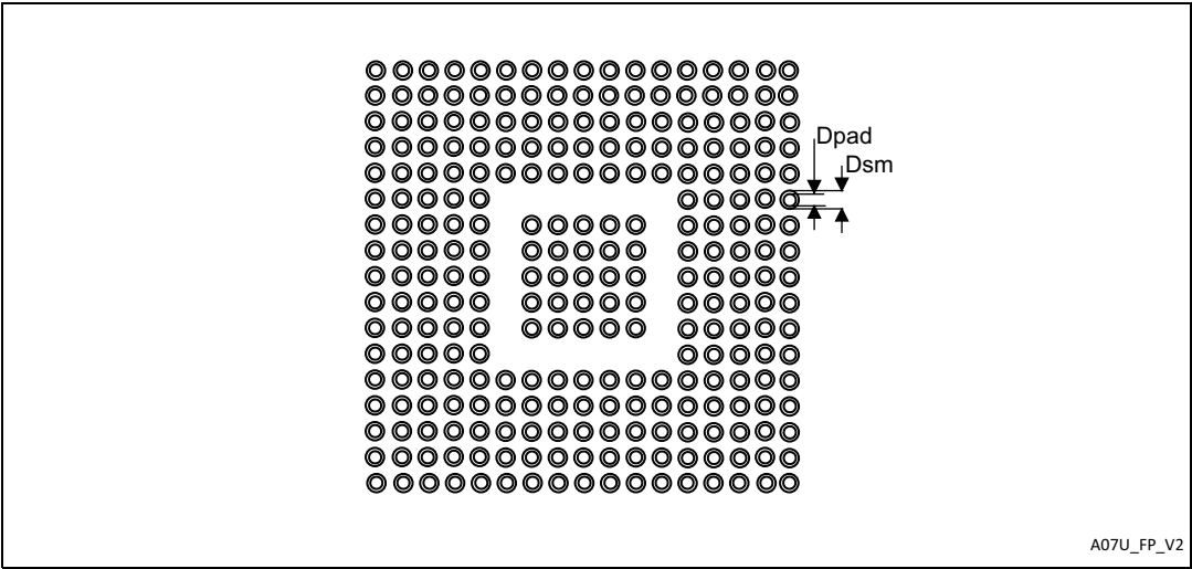
Figure 141. TFBGA240+25 package recommended footprint
