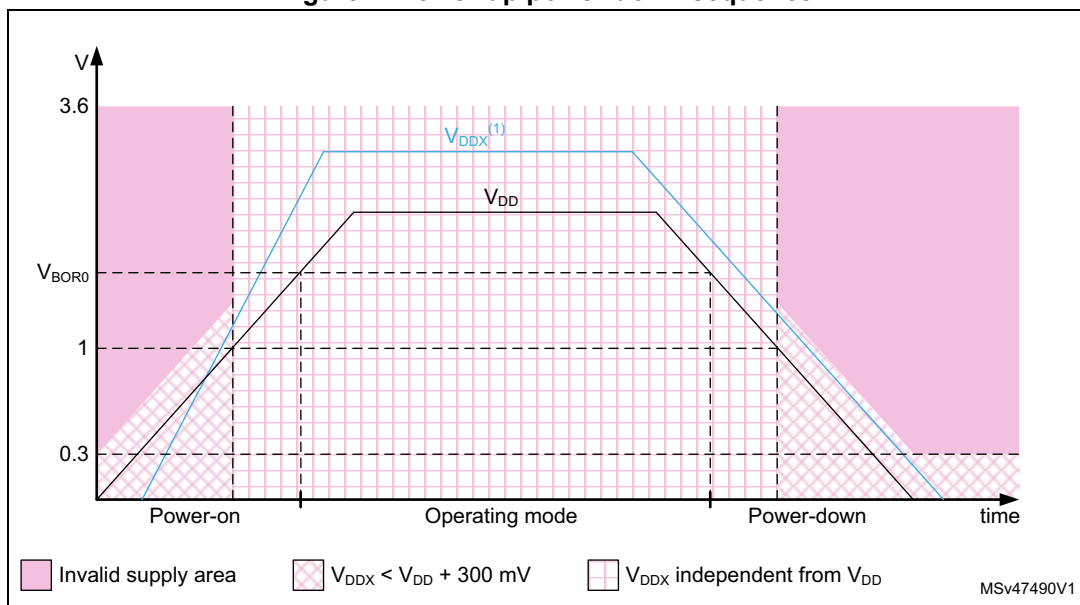
Figure 4. Power-up/power-down sequence
