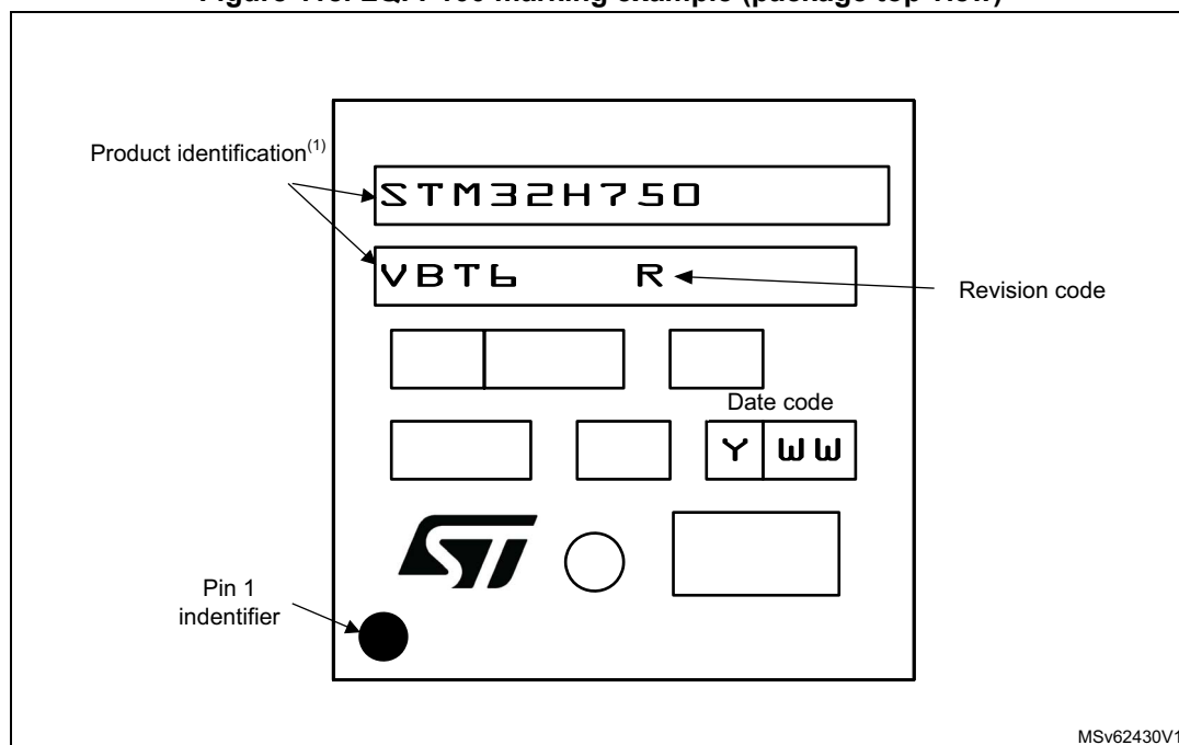
Figure 118. LQFP100 marking example (package top view)
