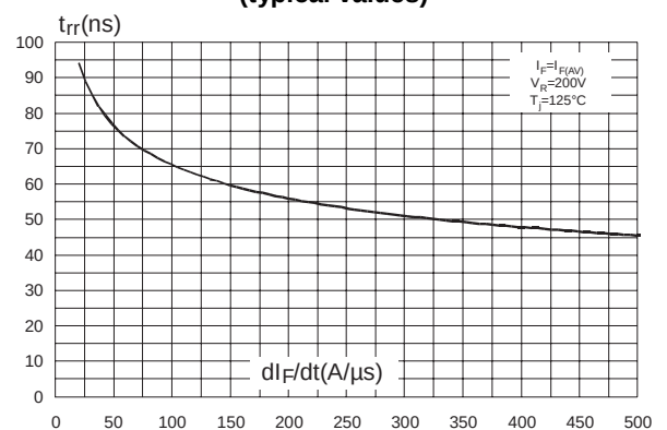
Figure 6: Reverse recovery time versus di/dt (typical values)
