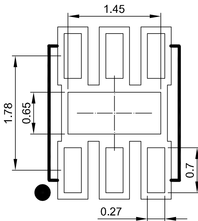
Figure 10. Landing pattern
