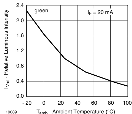
Figure 20. Relative Luminous Intensity vs. Amb. Temperature
