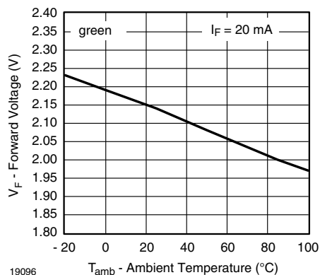
Figure 21. Forward Voltage vs. Ambient Temperature
