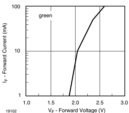
Figure 22. Forward Current vs. Forward Voltage
