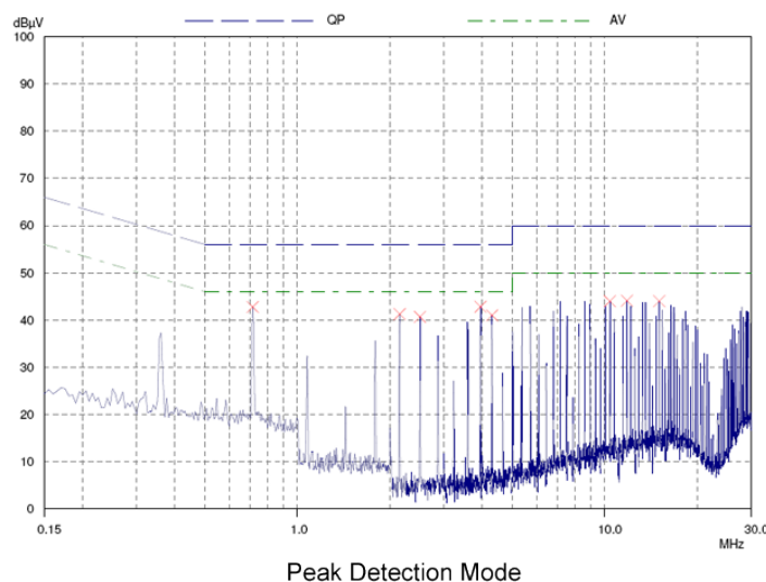
Graph 1. Conducted emissions performance, CISPR/EN55022, Class B, full load, filtered
