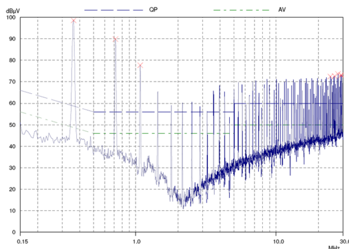
Graph 1. Conducted emissions performance, CISPR/EN55022, Class B, full load, unfiltered
